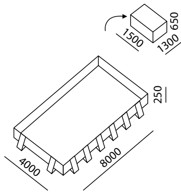
Dimensional ratio of staggered and folded tank
